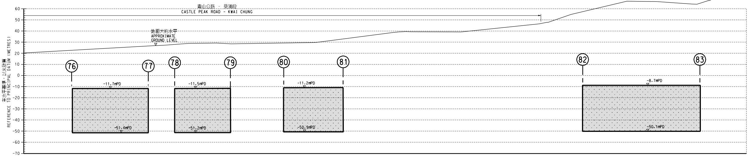
沿參線的剖面立視圖 SECTIONAL ELEVATION ALONG REFERENCE LINE
