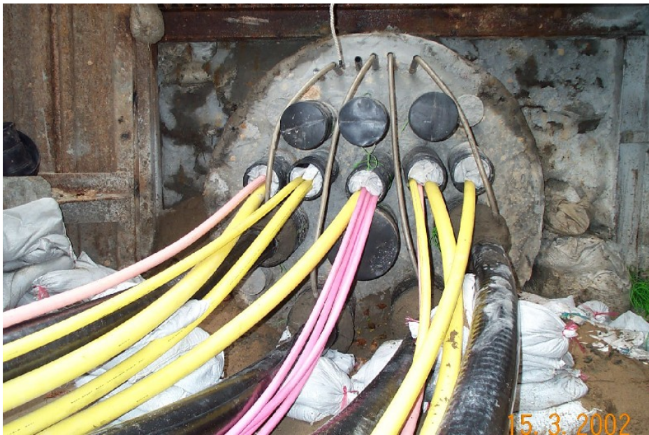
Photo 8 – 132kV Cable Ducts
