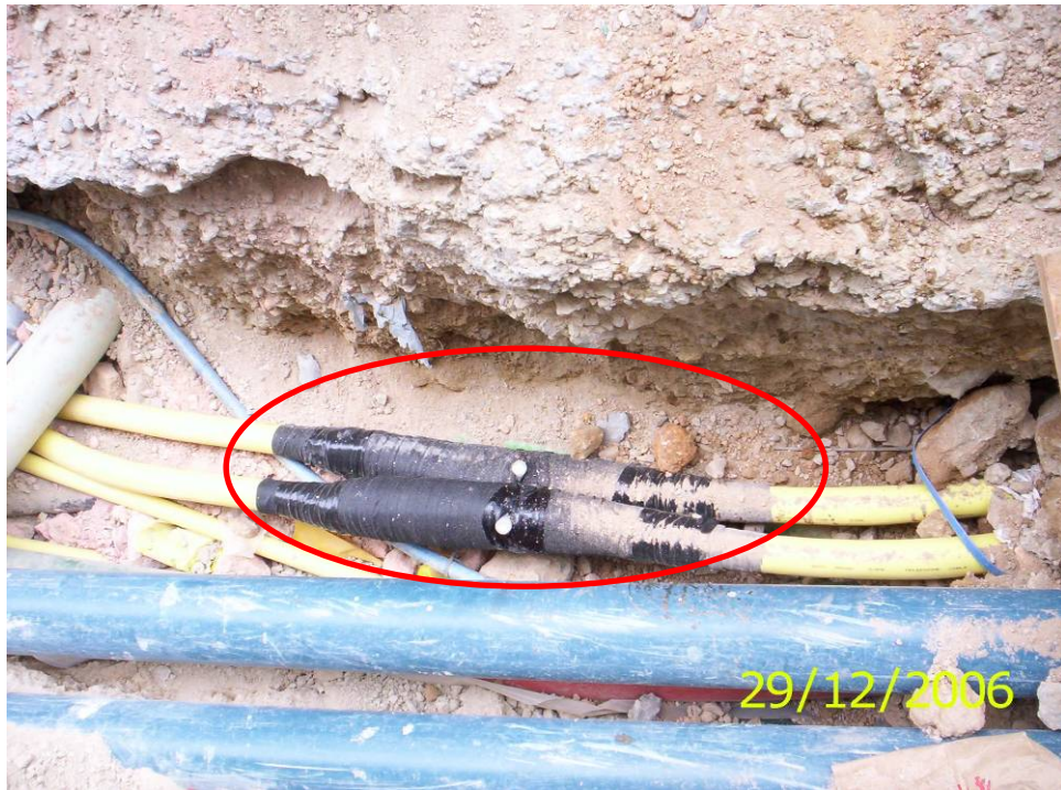
Photo 13 – Pilot Cable Joints
