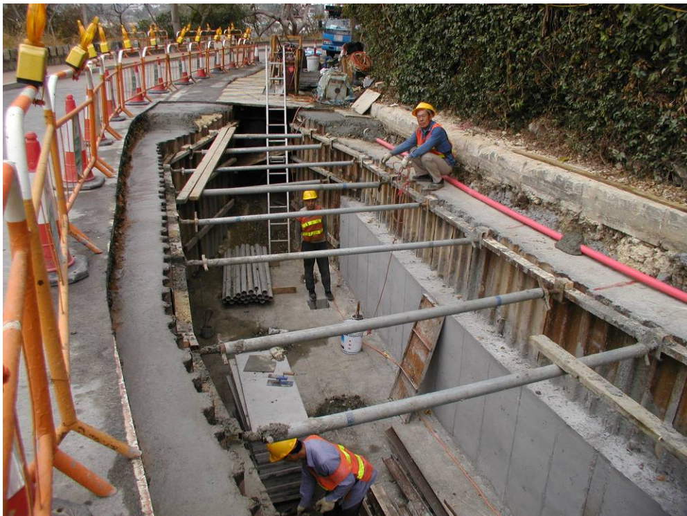
Photo 20 – Transmission Cable Joint Bay
