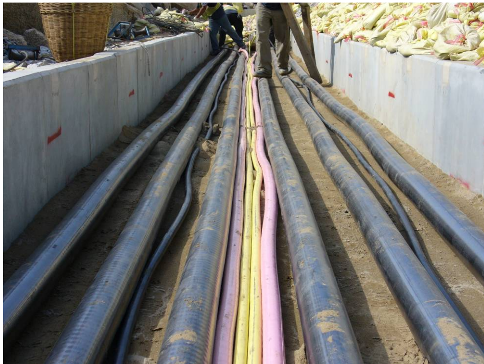
Photo 10 – 275kV Cables
