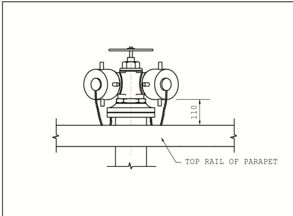
FIG.5 - RAISING OF FIRE HYDRANT ON ELEVATED HIGHWAY STRUCTURES TO AVOID OBSTRUCTION
