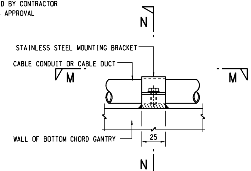
DETAIL 12 SCALE 1:2
