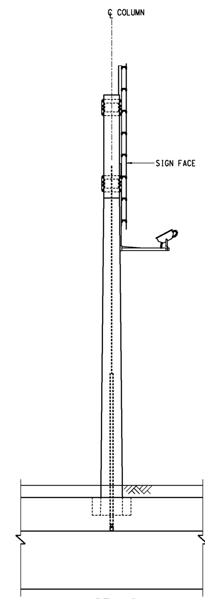
VIEW C SCALE 1:50
