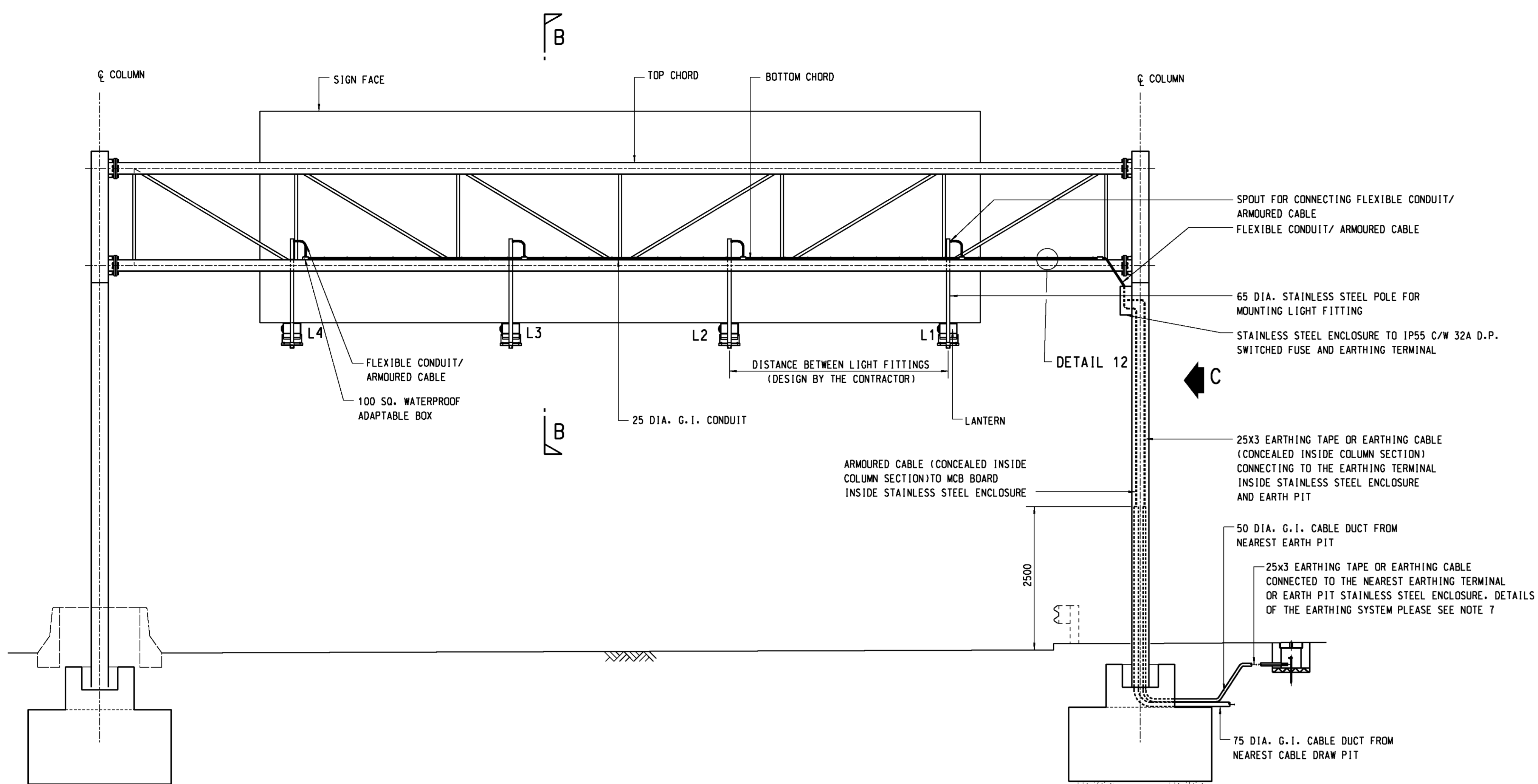
REAR ELEVATION SIGN POST NOT SHOWN FOR CLARITY SCALE 1:50
