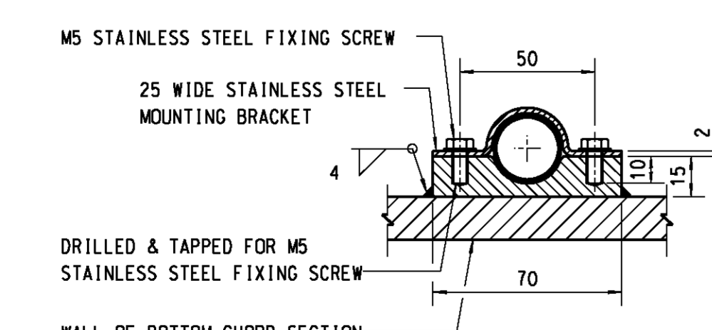
SECTION N-N SCALE 1:2
