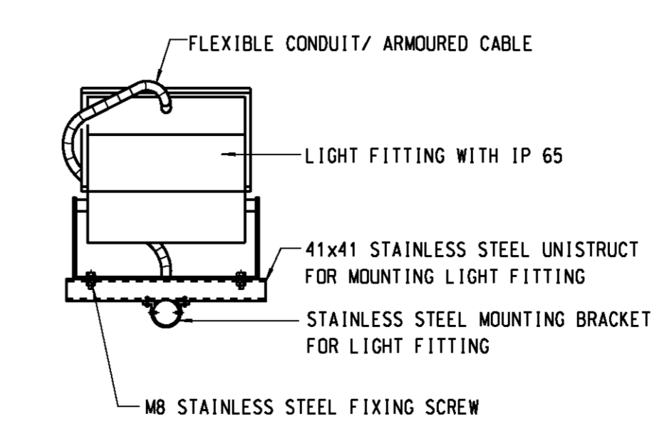
ELEVATION Q-Q SCALE 1:10
