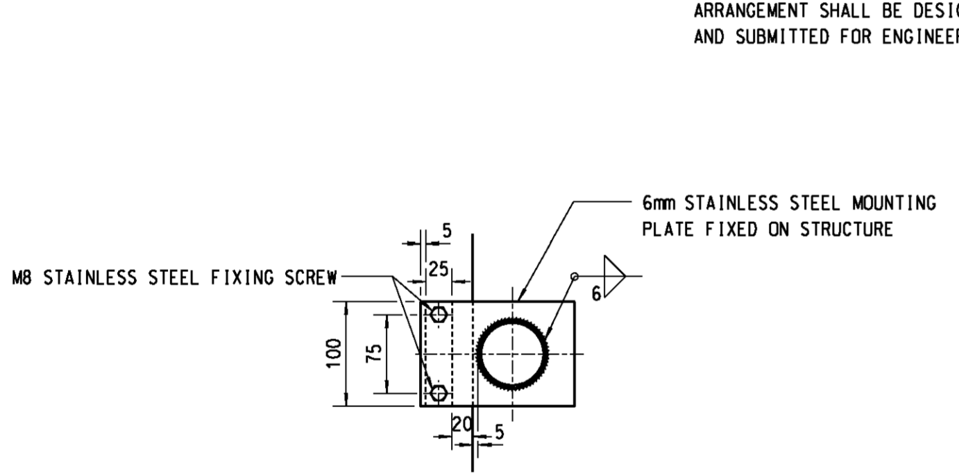
SECTION L-L SCALE 1:5
