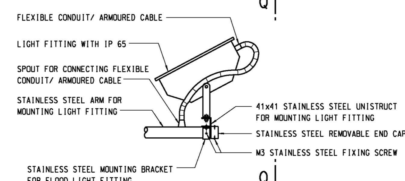
DETAIL 15 SCALE 1:10
