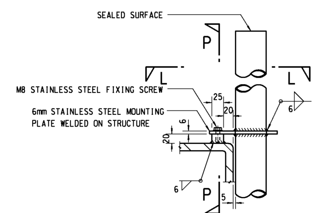
DETAIL 13 SCALE 1:5
