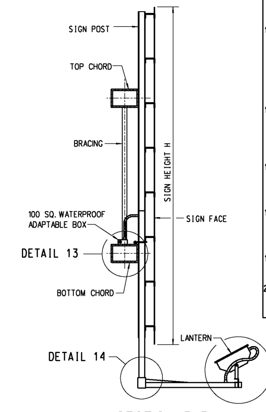
SECTION B-B SCALE 1:25
