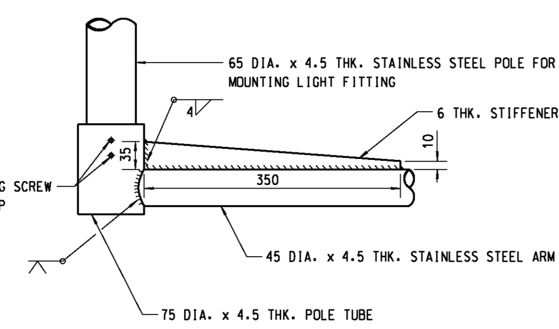
DETAIL 14 SCALE 1:5
