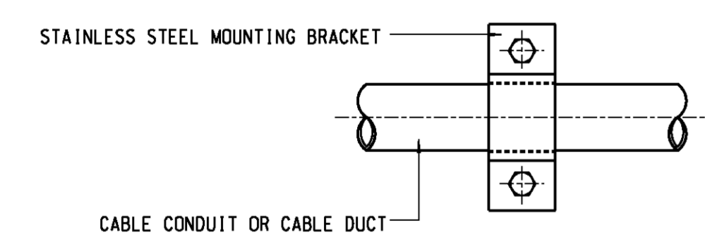
PLAN M-M SCALE 1:2
