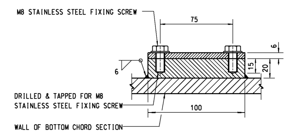
SECTION P-P SCALE 1:2
