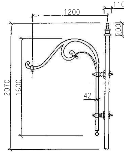
BRACKET (TYPE B)
