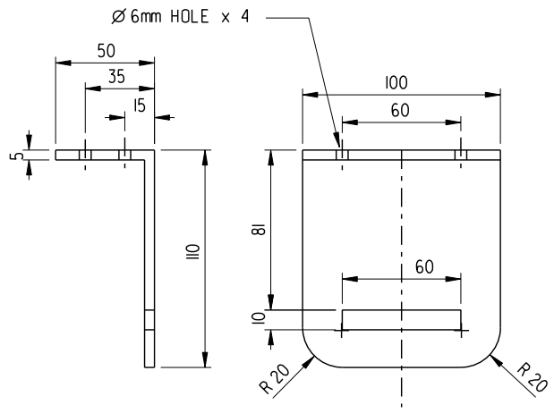
END VIEW BACK PLATE
