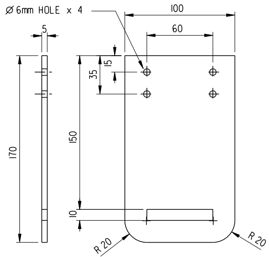
END VIEW FRONT PLATE
