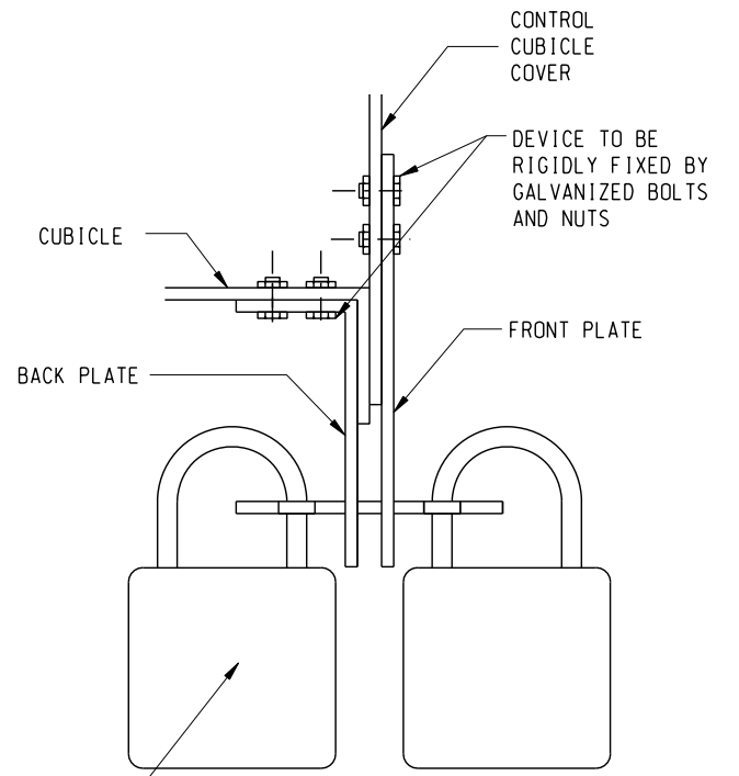
ASSEMBLY SECTIONAL VIEW
