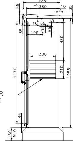
SIDE VIEW ON ARROW B
