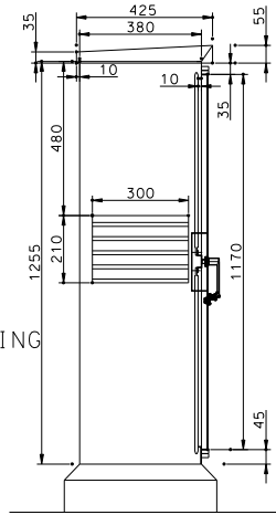
SIDE VIEW ON ARROW A
