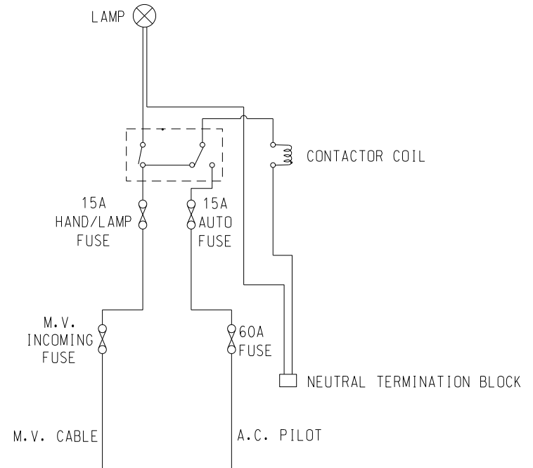
CONTROL WIRING SCHEMATIC
