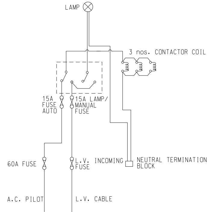
CONTROL WIRING SCHEMATIC
