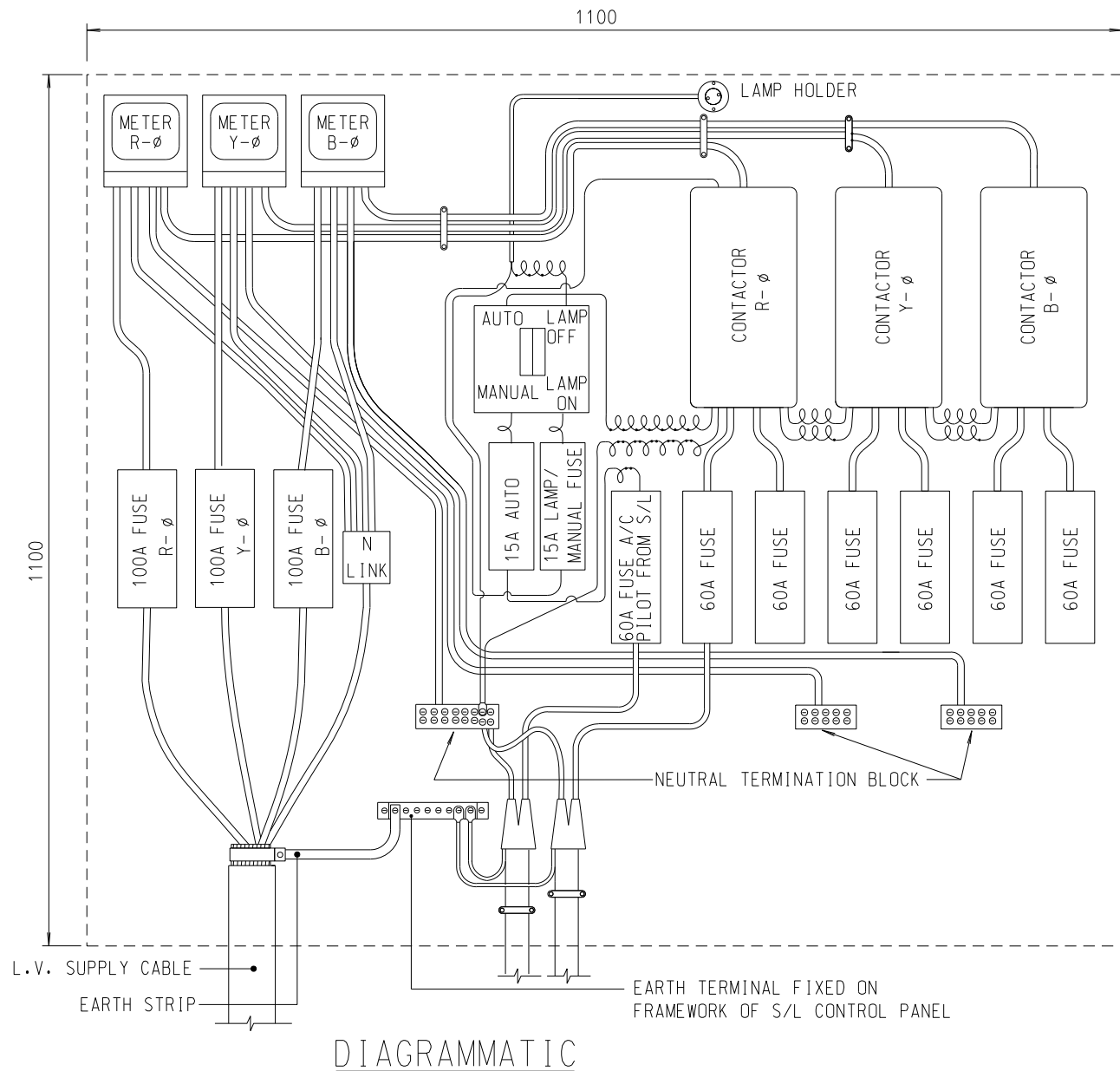
CONTROL WIRING SCHEMATIC
