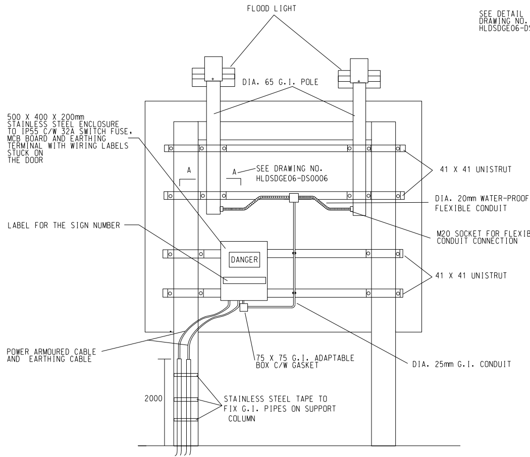
TYPICAL INSTALLATION DETAIL (FOR REFERENCE ONLY) VIEW A
