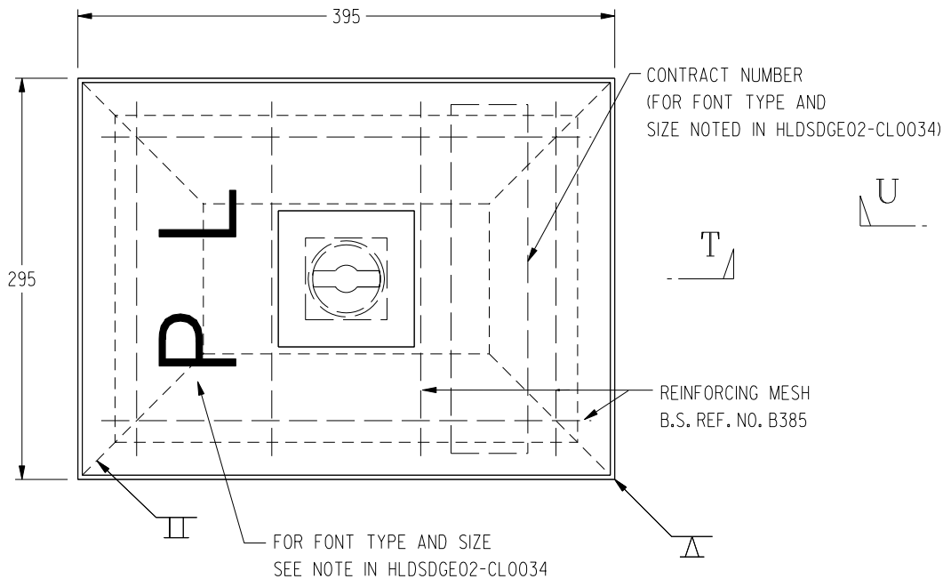
PLAN (COVER)
