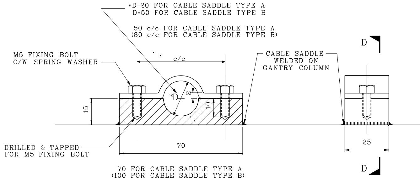
DETAIL 'C' (FOR CABLE SADDLE TYPE A & B)
