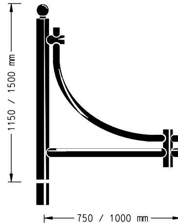
TYPE C BRACKET
