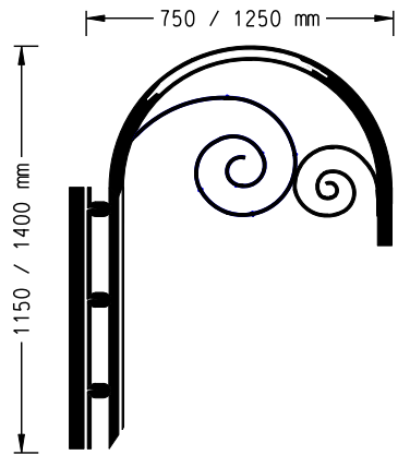
TYPE A BRACKET
