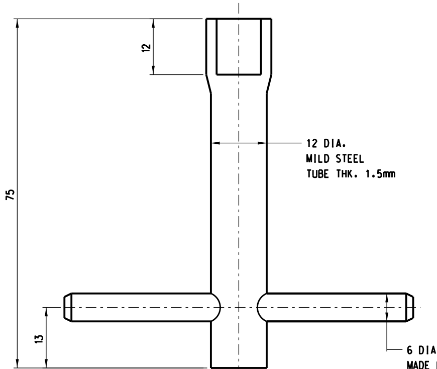
FRONT ELEVATION
