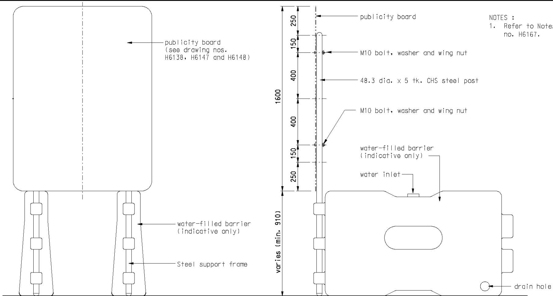
FRONT ELEVATION
