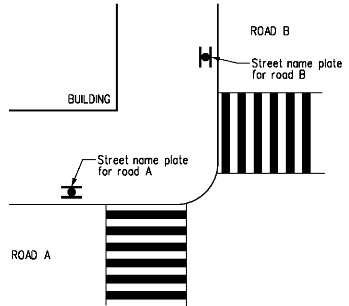
LAYOUT FOR CENTRE-MOUNTED STREET NAME PLATES IN THE PRESENCE OF PEDESTRIAN CROSSING
