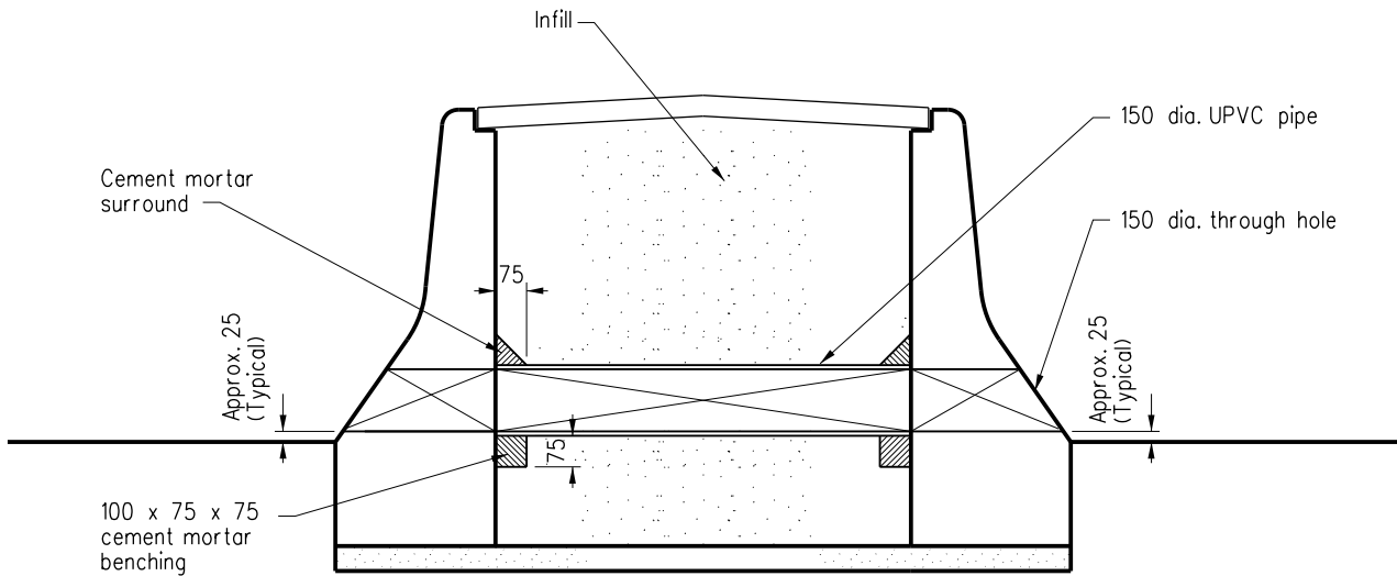
TYPICAL CROSS SECTION FOR DRAIN HOLES ACROSS DOUBLE-SIDED CENTRAL DIVIDER
