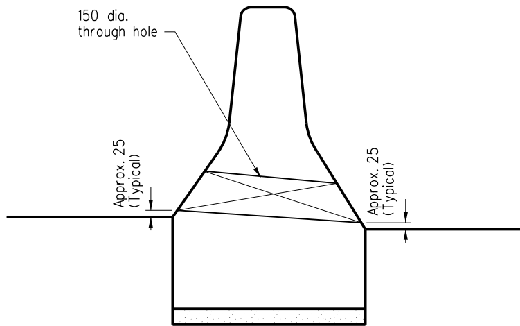
TYPICAL CROSS SECTION FOR DRAIN HOLES ACROSS SINGLE CENTRAL DIVIDER
