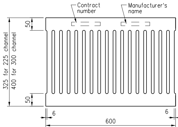
GRATING
