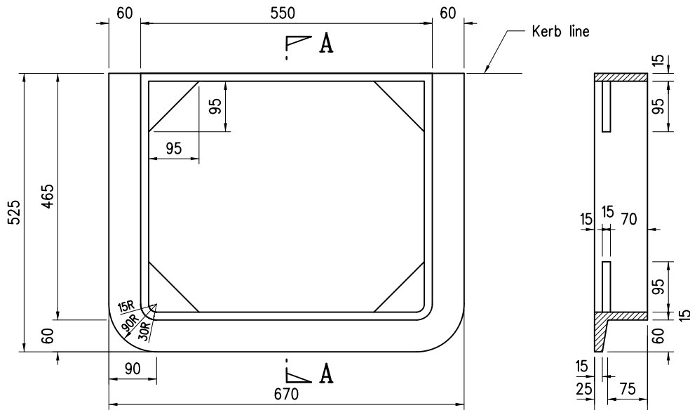
FRAME (For Gully Grating Adjacent to Kerb)
