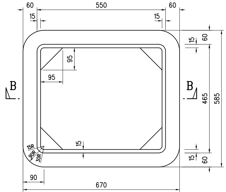
FRAME (For Gully Grating Away from Kerb)
