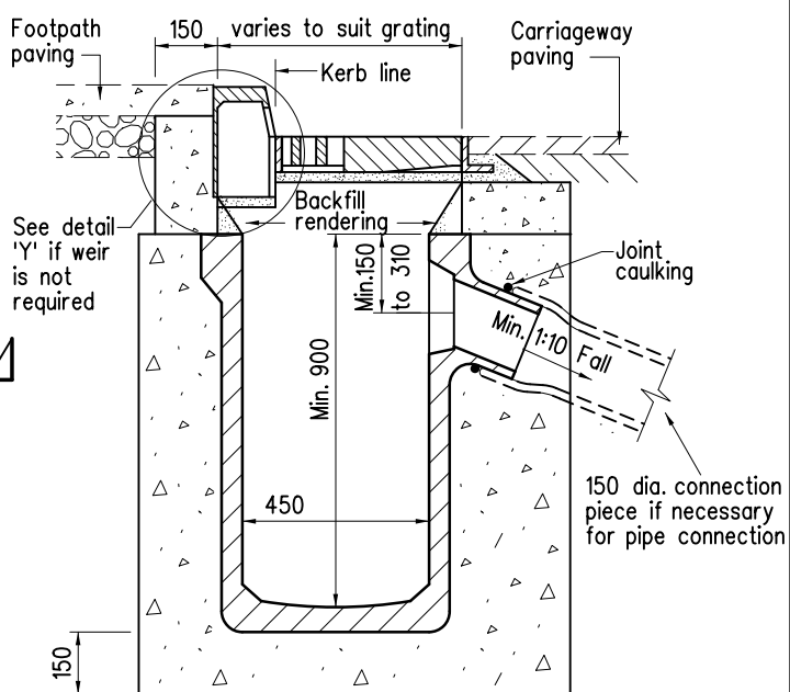
SECTION B-B
