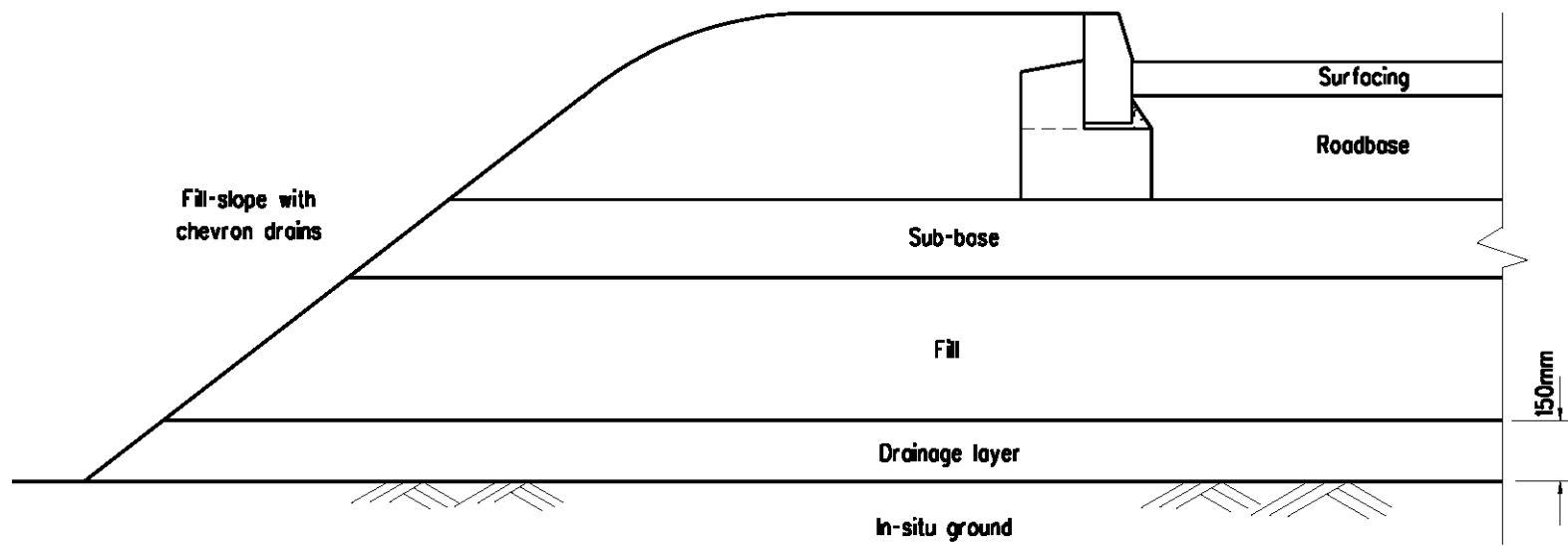
CROSS - SECTION
