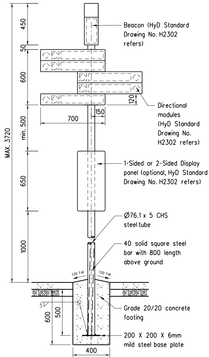
SECTION VIEW
