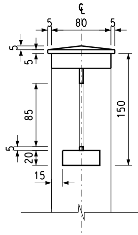
SECTION E-E SCALE 1:5
