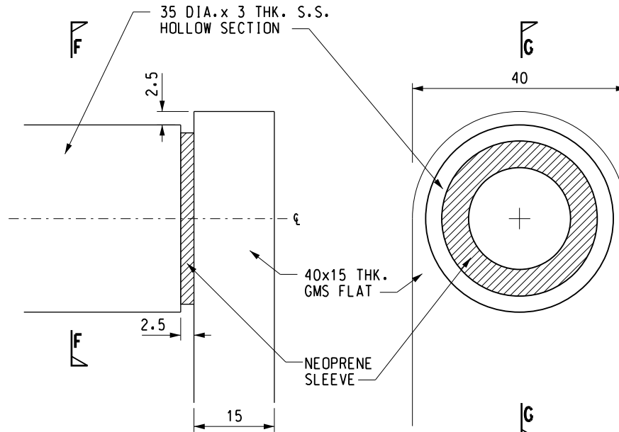
DETAIL 'Z'
