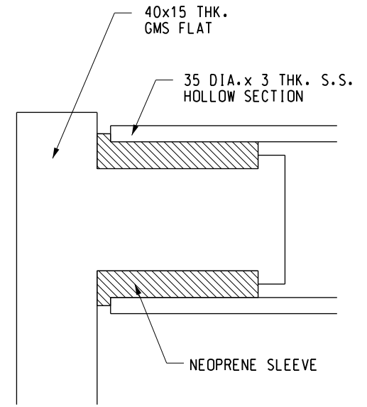
SECTION G-G
