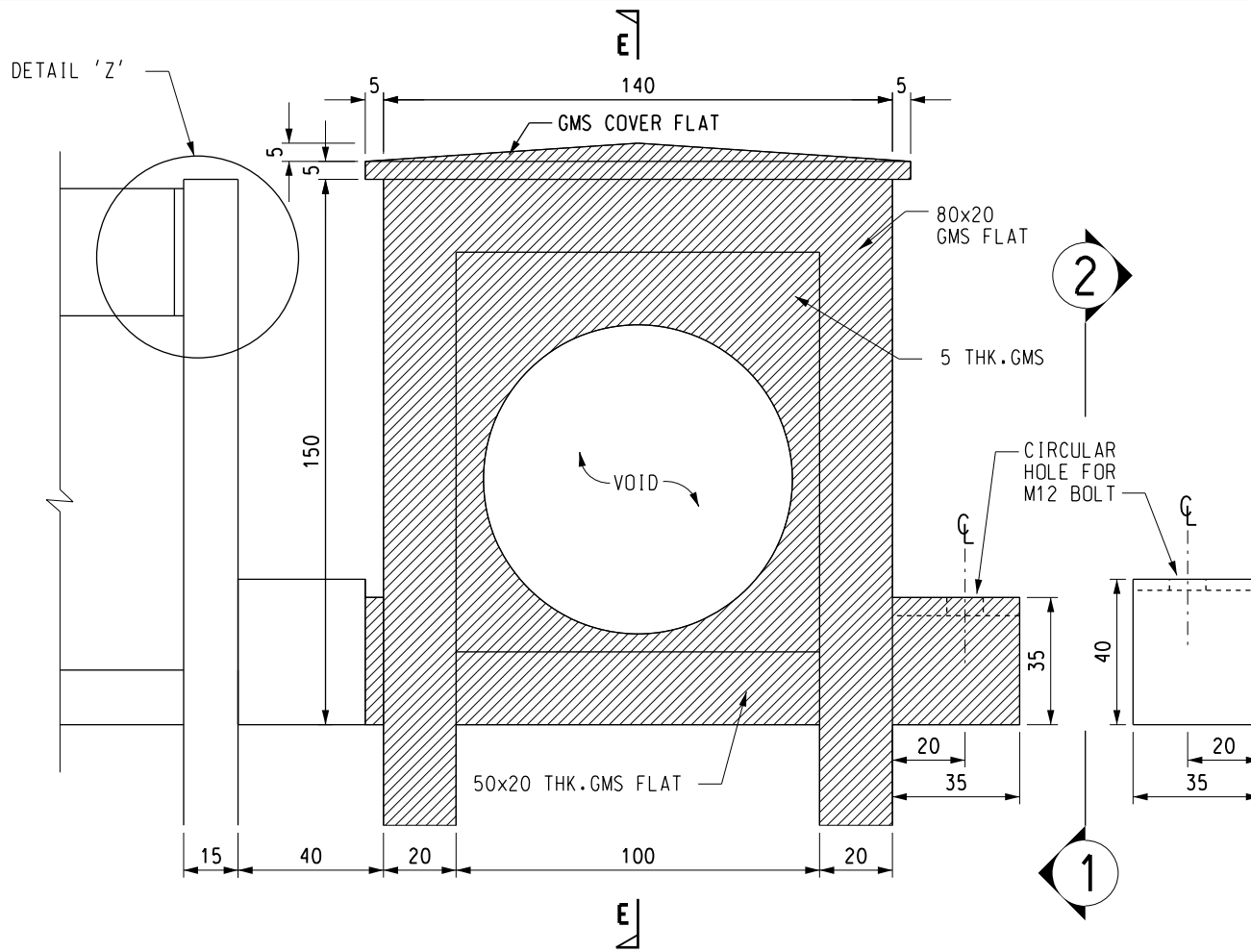
DETAIL 'Y' (TYPICAL CONNECTION BETWEEN POST & PANELS)
