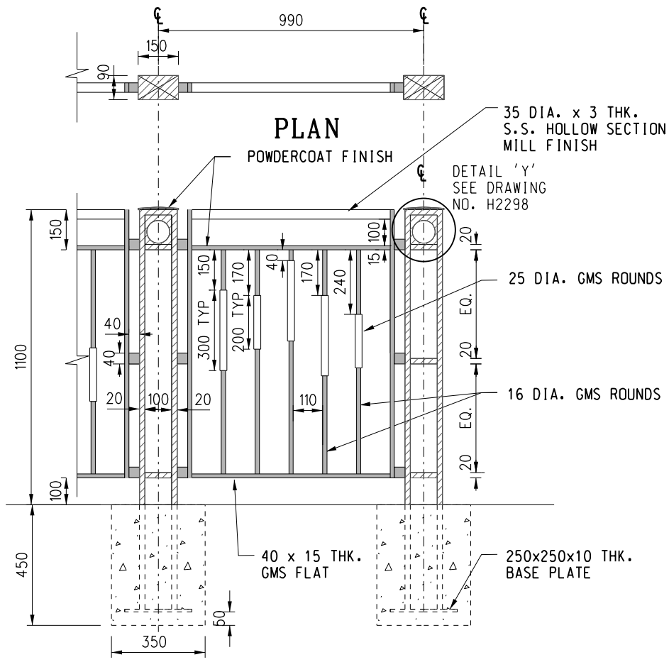
SECTIONAL ELEVATION
