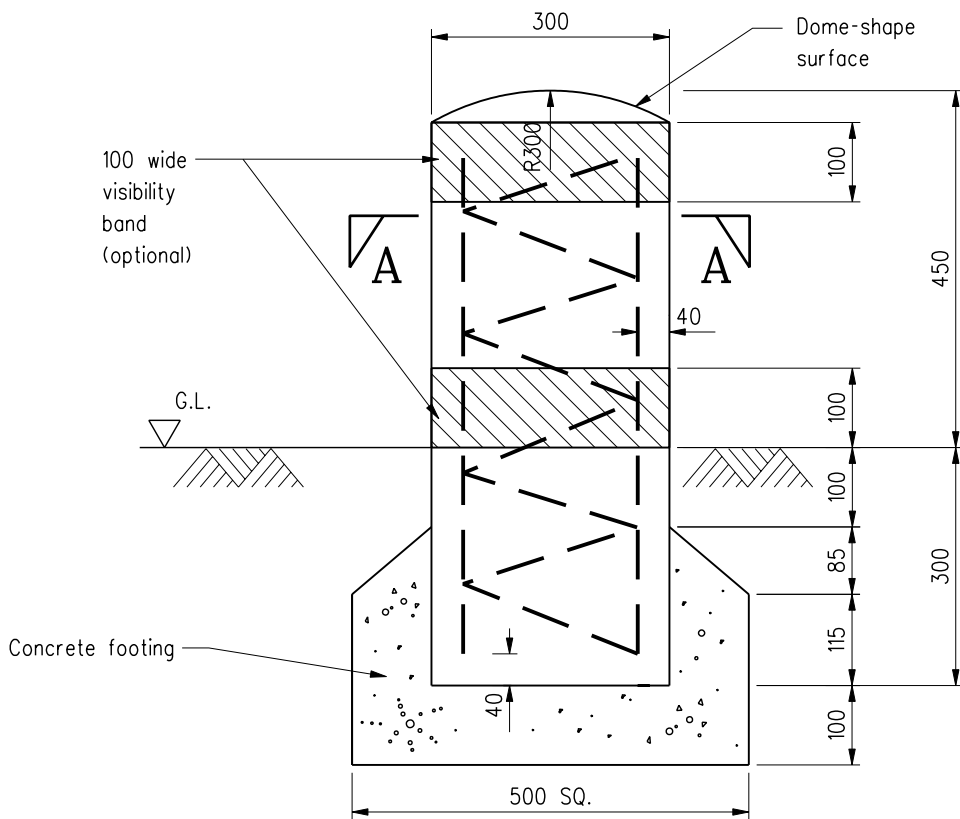
SECTION - ELEVATION
