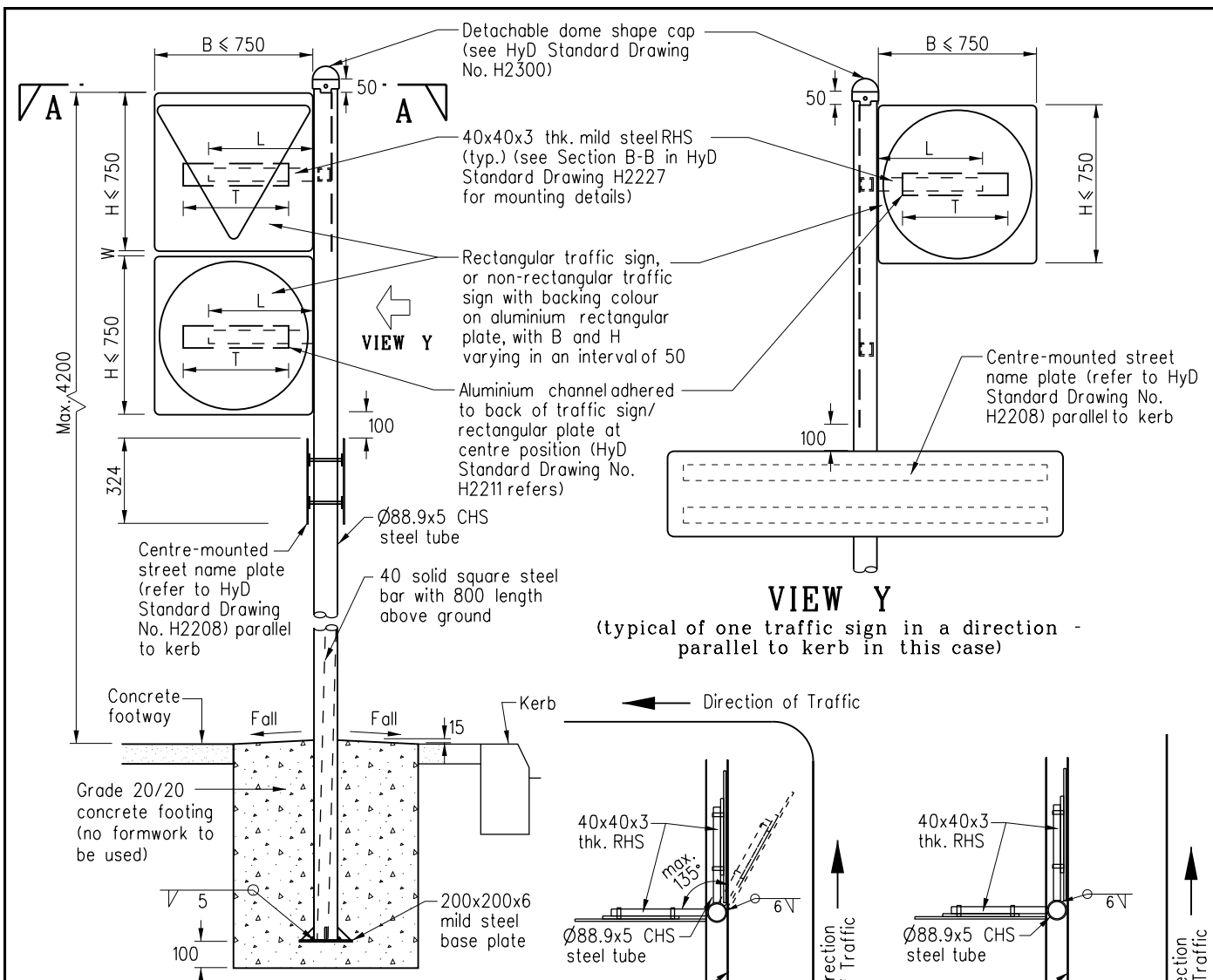
FRONT ELEVATION (VIEW X) (typical of two traffic signs in a direction - perpendicular to kerb in this case)
