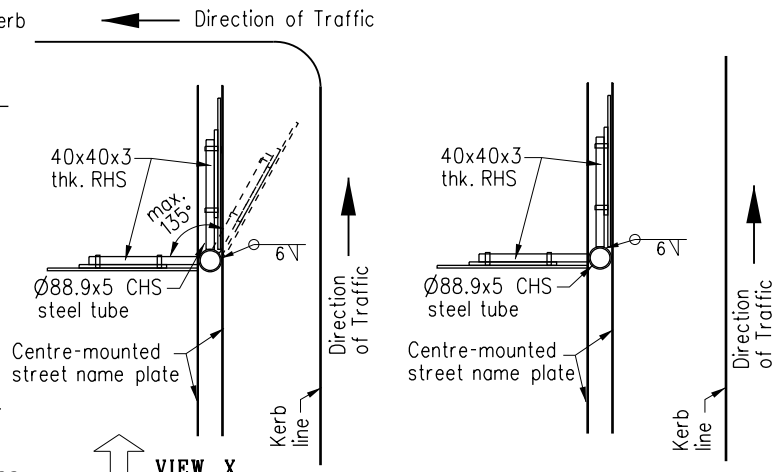
SECTION A-A (position at road junction)
