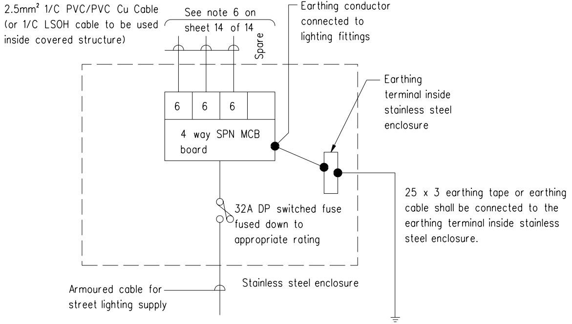
TYPICAL SCHEMATIC WIRING DIAGRAM ( HEIGHT OF SIGN FACE 1m TO 4m )
