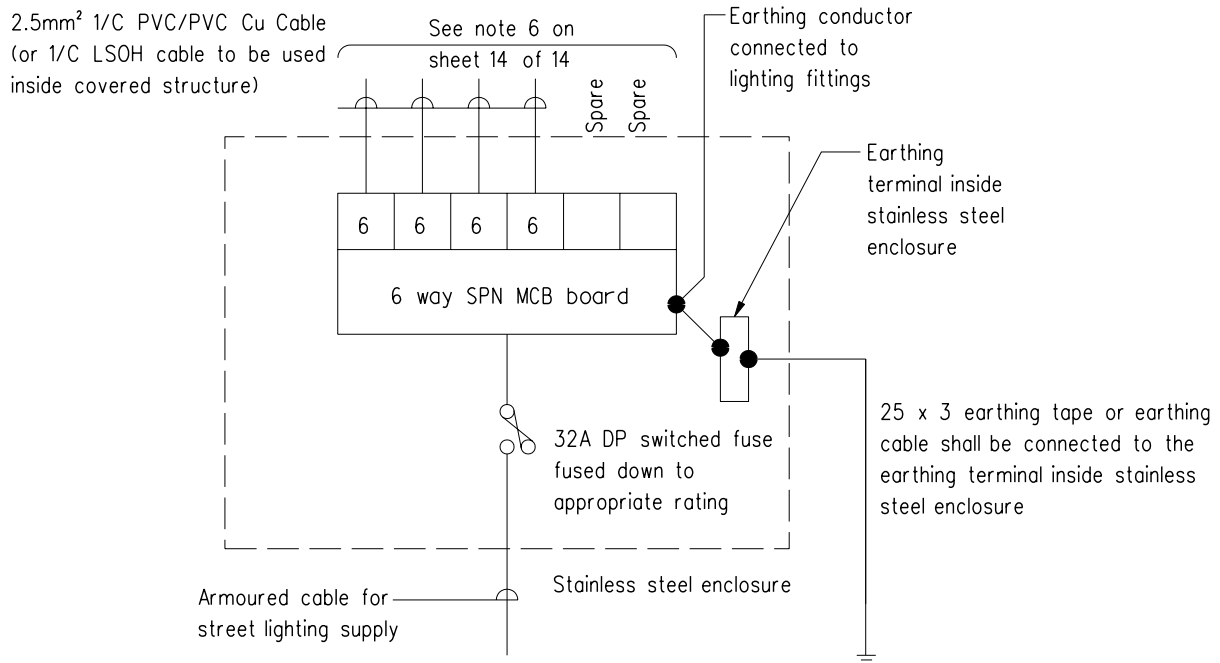
TYPICAL SCHEMATIC WIRING DIAGRAM ( HEIGHT OF SIGN FACE GREATER THAN 4m )
