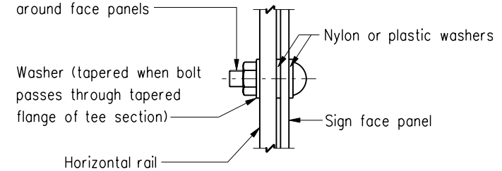
DETAIL 4
