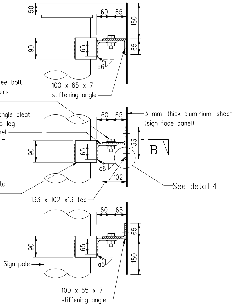
TYPICAL CONNECTION OF SIGN FACE PANEL TO SUPPORTING POLES
