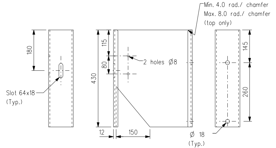
ELEVATIONS
