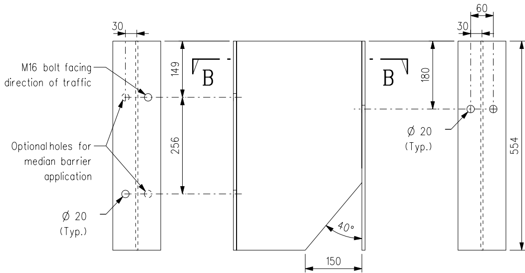
ELEVATIONS
