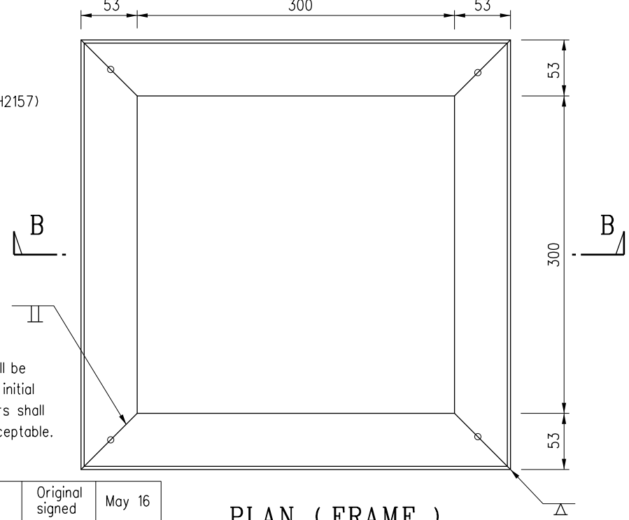
PLAN ( FRAME )
