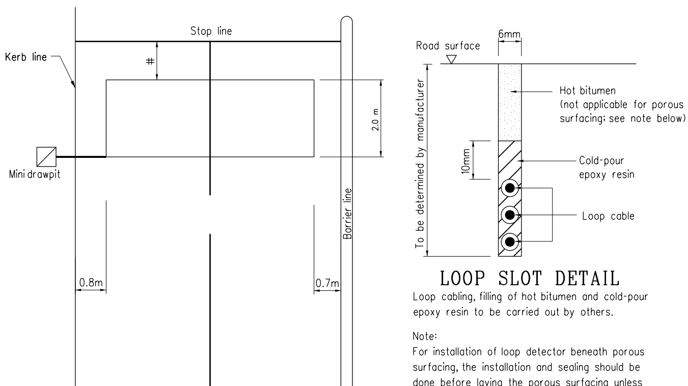
LOOP LAYOUT FOR TACTICAL DETECTION
