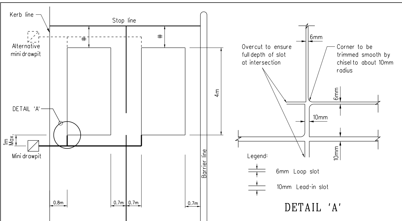
LOOP LAYOUT FOR STRATEGIC DETECTION
