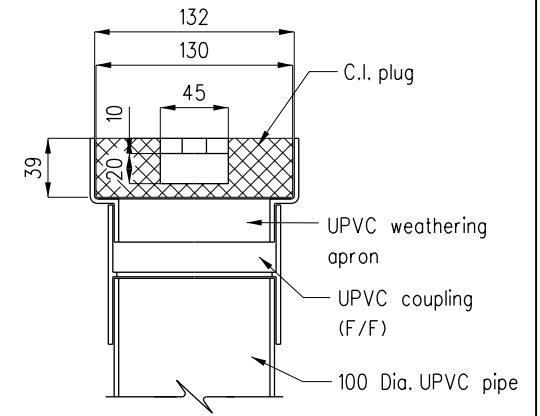
SECTIONAL VIEW
