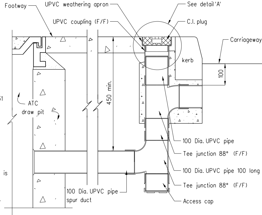
SECTION W - W (For cable connecting detector loops on c/w)
