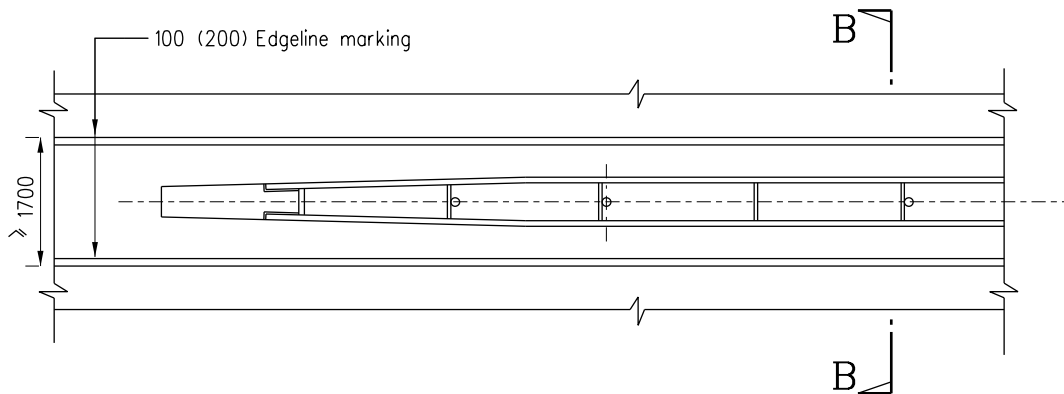
PLAN FOR WIDE CENTRAL RESERVATION WITH ANCHOR BLOCK AND HORIZONTAL FLARE
