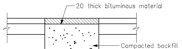
Temporary reinstatement
