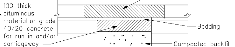
Temporary reinstatement
