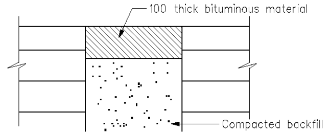
Temporary reinstatement
