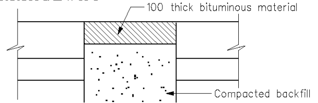
Temporary reinstatement
