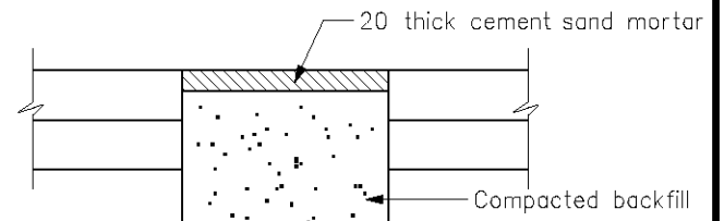
Temporary reinstatement
