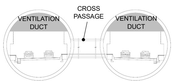
TYPICAL SECTION OF THE PROPOSED VEHICULAR TUNNEL
