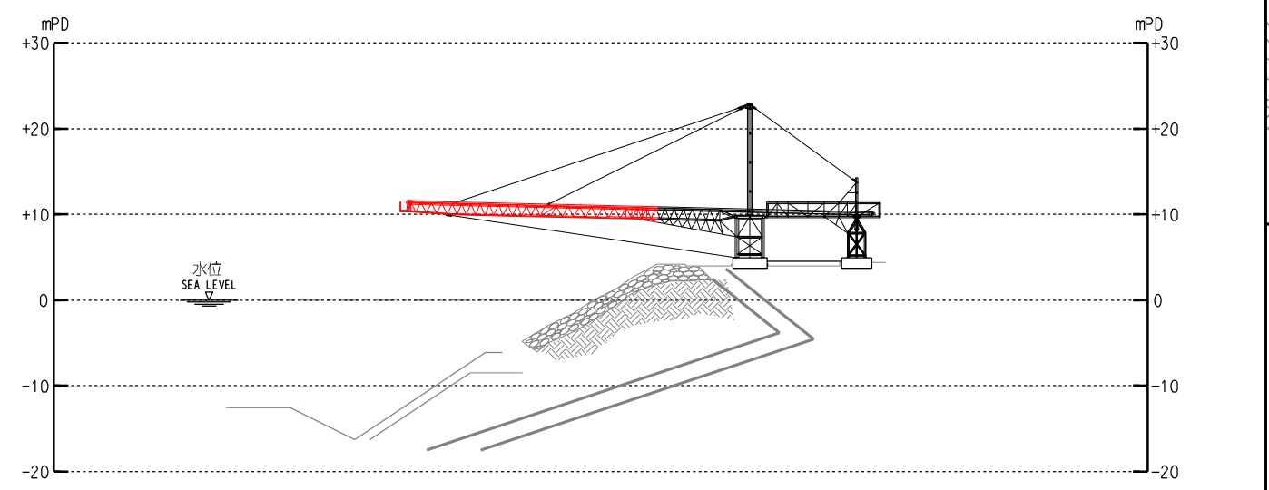
躉船起卸台的典型切面圖 TYPICAL SECTION OF BARGE LOADING RAMP 不按比例 NOT TO SCALE
