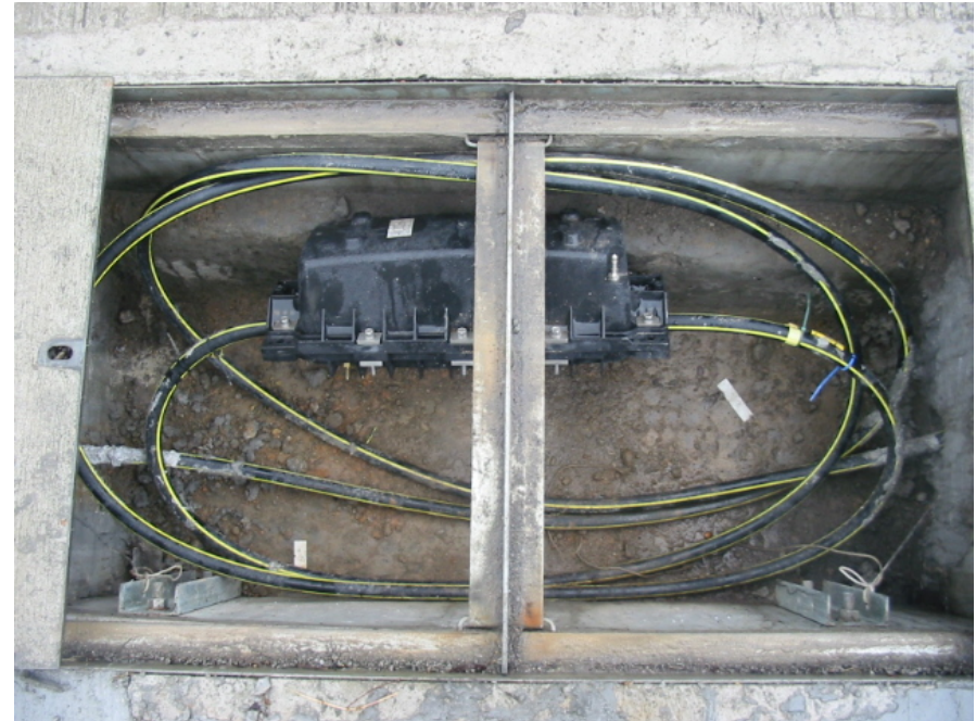
Photo 2 – Cable and Cable Joint (NWT)
