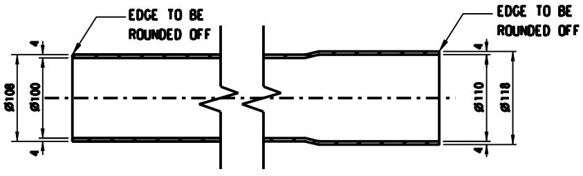
DETAIL 'A' (UPVC) DETAIL 'B'
