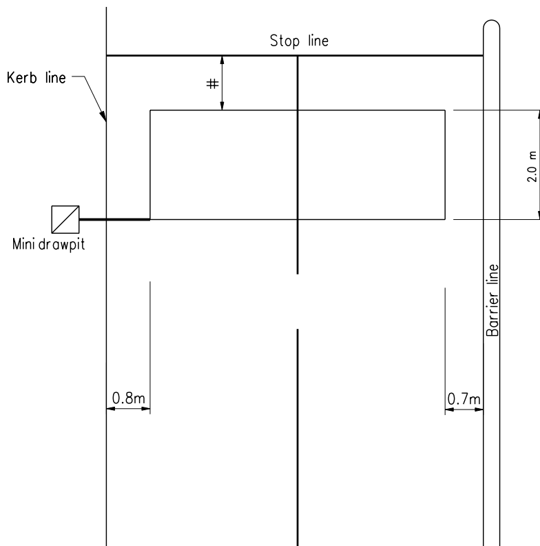
LOOP LAYOUT FOR TACTICAL DETECTION
