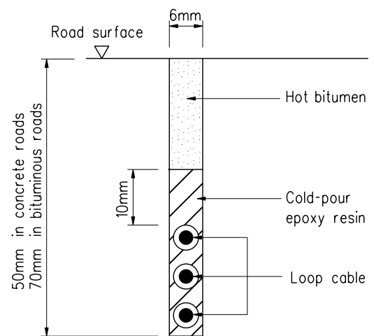
LOOP SLOT DETAIL
