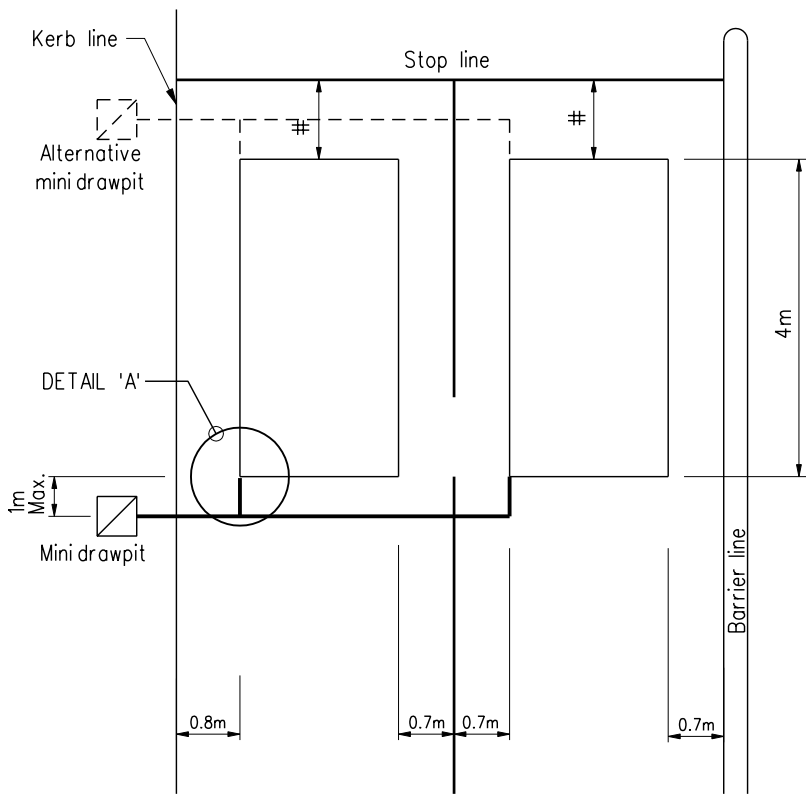
LOOP LAYOUT FOR STRATEGIC DETECTION
