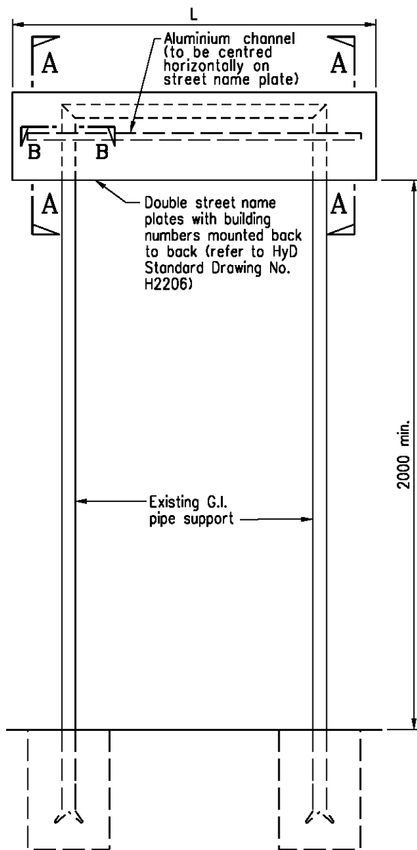
FRONT ELEVATION
