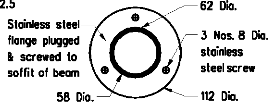
SECTION G - G
