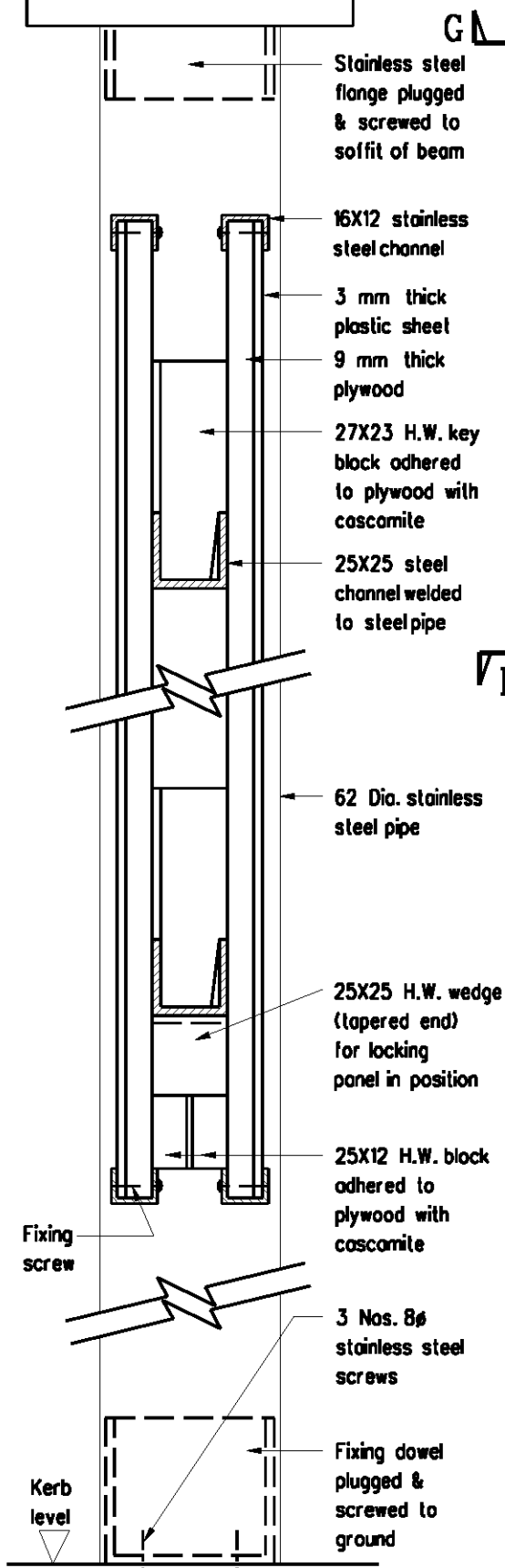
SECTIONAL VIEW
