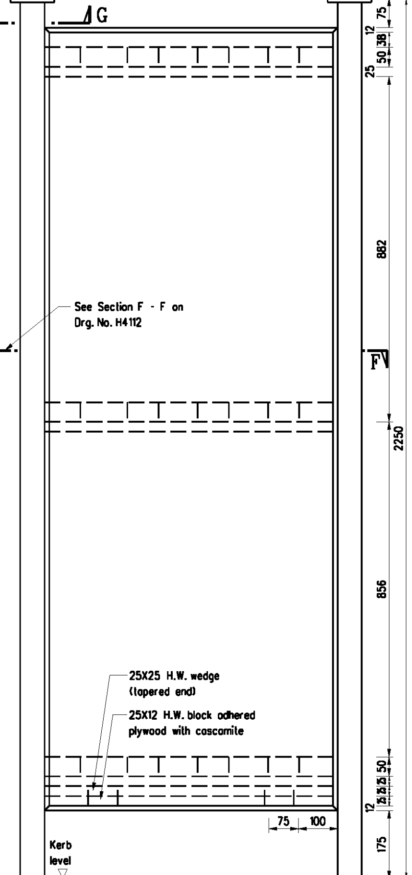
ELEVATION Scale 1 : 10
