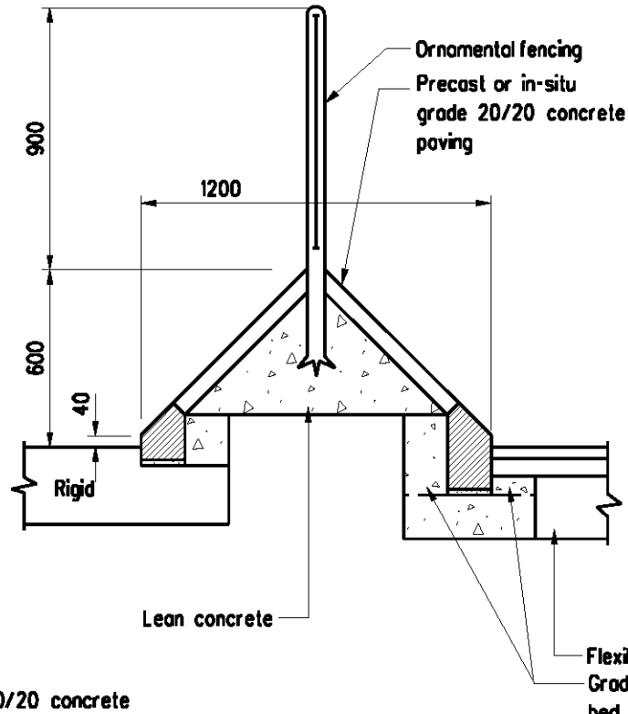
TRIANGULAR 40 UPSTAND
