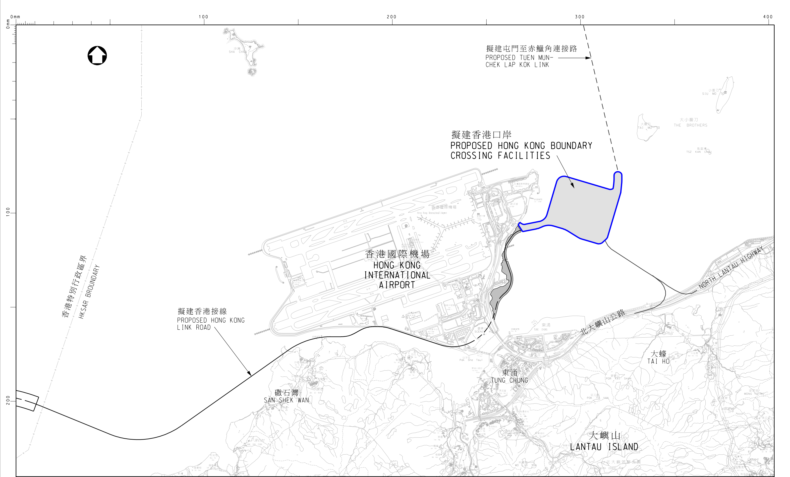
港珠澳大橋香港口岸首選方案 HONG KONG BOUNDARY CROSSING FACILITIES FOR HONG KONG - ZHUHAI - MACAO BRIDGE PREFERRED OPTION
